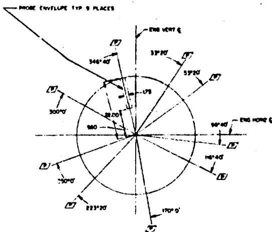
SCHEMATIC VIEW LOOKING FORWARD AT PLANE (D) (P-1) TURBINE ENT TEMPERATURE THERMOCOUPLES AT LOC INDICATED BY (E)
